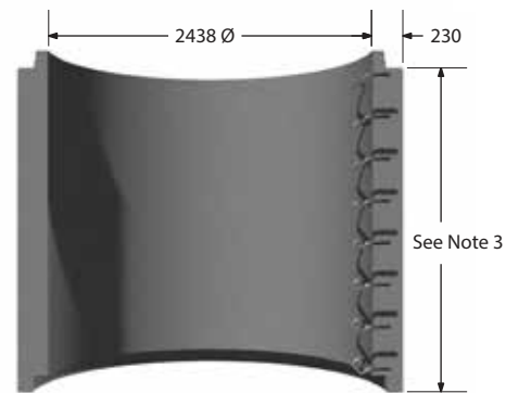
Section B-B
